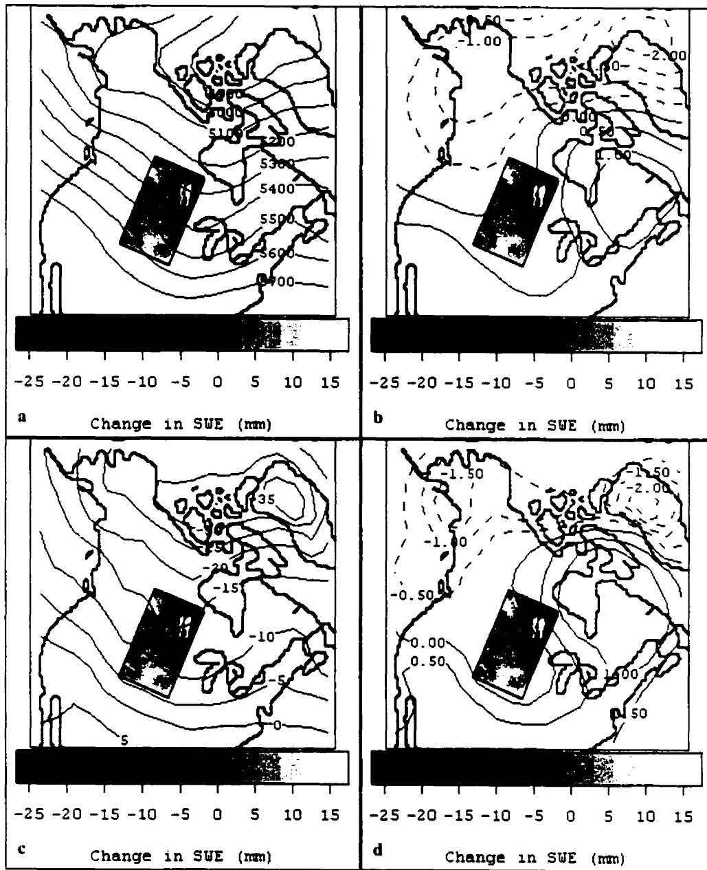
Figure 7.19 500Z composite (a) and anomaly (b), and 700T composite (c) and anomaly (d) fields, which correspond to the negative phase of \Delta\text{SWE PC4} .
