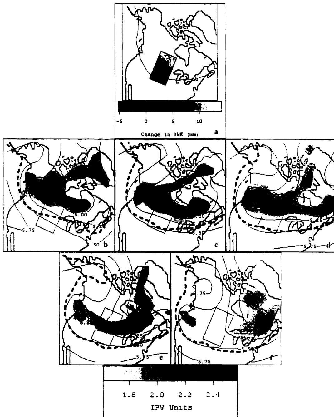
Figure 7.50 \Delta SWE PC1+ (shown in a with pentad average -10^{\circ}\text{C} isotherm at 700 mb) case study. Daily data for Jan. 31 ( b ) 1989 through Feb. 4 ( f ) 1989 is shown. Gray tones illustrate IPV, the dashed line indicates the position of the -10^{\circ}\text{C} isotherm at 700 mb. solid lines depict the 500 mb geopotential height pattern (metres \bullet 10^3 ). \Delta SWE loading for this pentad is 0.72.
