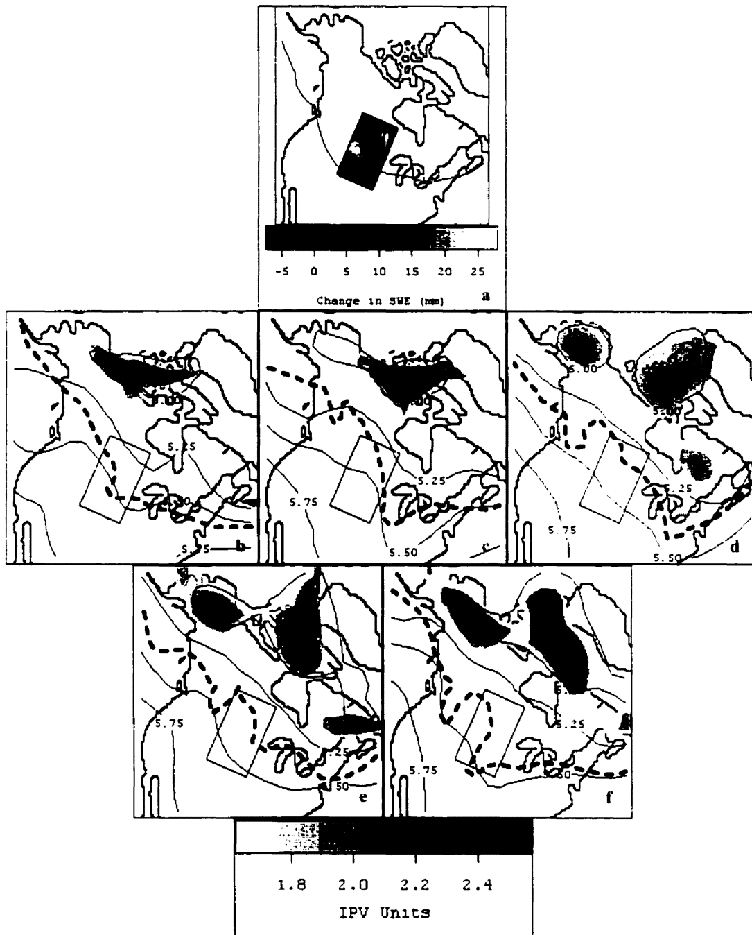
Figure 7.55 \Delta SWE PC3- (shown in a with pentad average -10^{\circ}\text{C} isotherm at 700 mb) case study. Daily data for Jan. 11 (b) 1989 through Jan. 15 (f) 1991 is shown. Gray tones illustrate IPV, the dashed line indicates the position of the -10^{\circ}\text{C} isotherm at 700 mb, solid lines depict the 500 mb geopotential height pattern (metres \cdot 10^3 ). \Delta SWE loading for this pentad is -0.55 .
