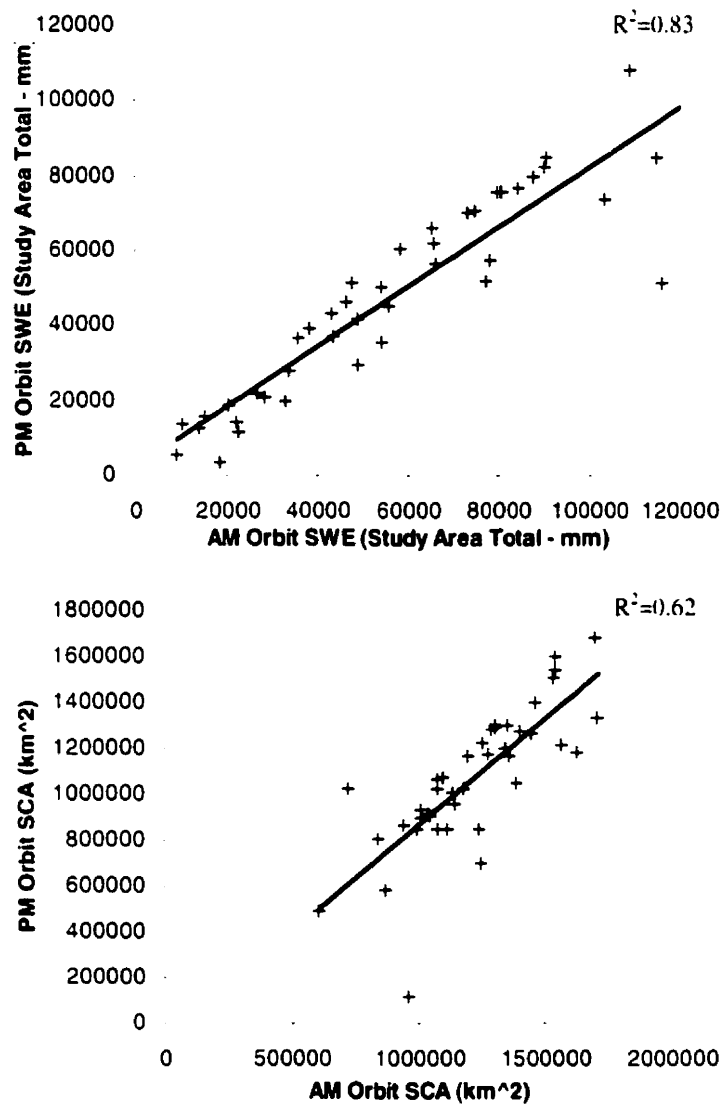
Figure 6.1 Correlation between AM and PM SWE (top) and SCA (bottom).
