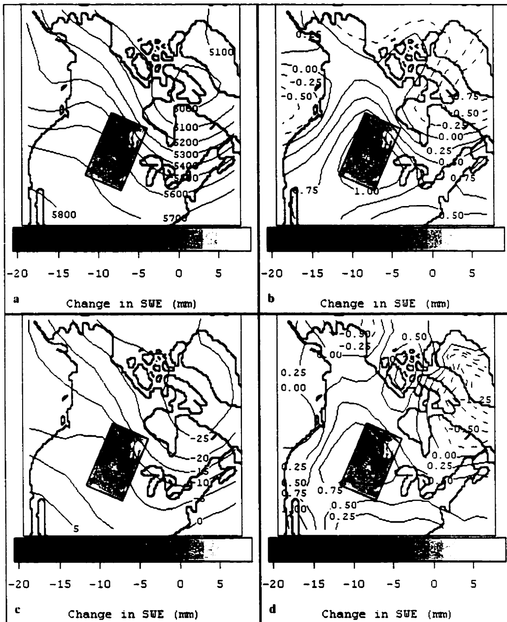
Figure 7.15 500Z composite (a) and anomaly (b), and 700T composite (c) and anomaly (d) fields, which correspond to the negative phase of \Delta\text{SWE PC2} .
