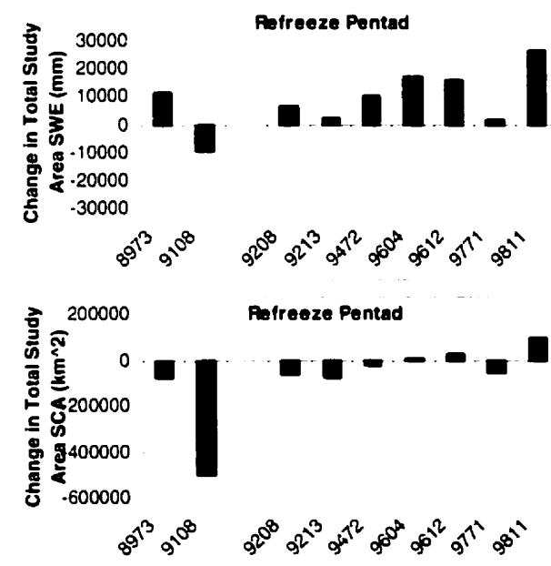
Figure 6.6 Change in total Prairie SWE (top) and SCA (bottom) for refreeze pentads.
