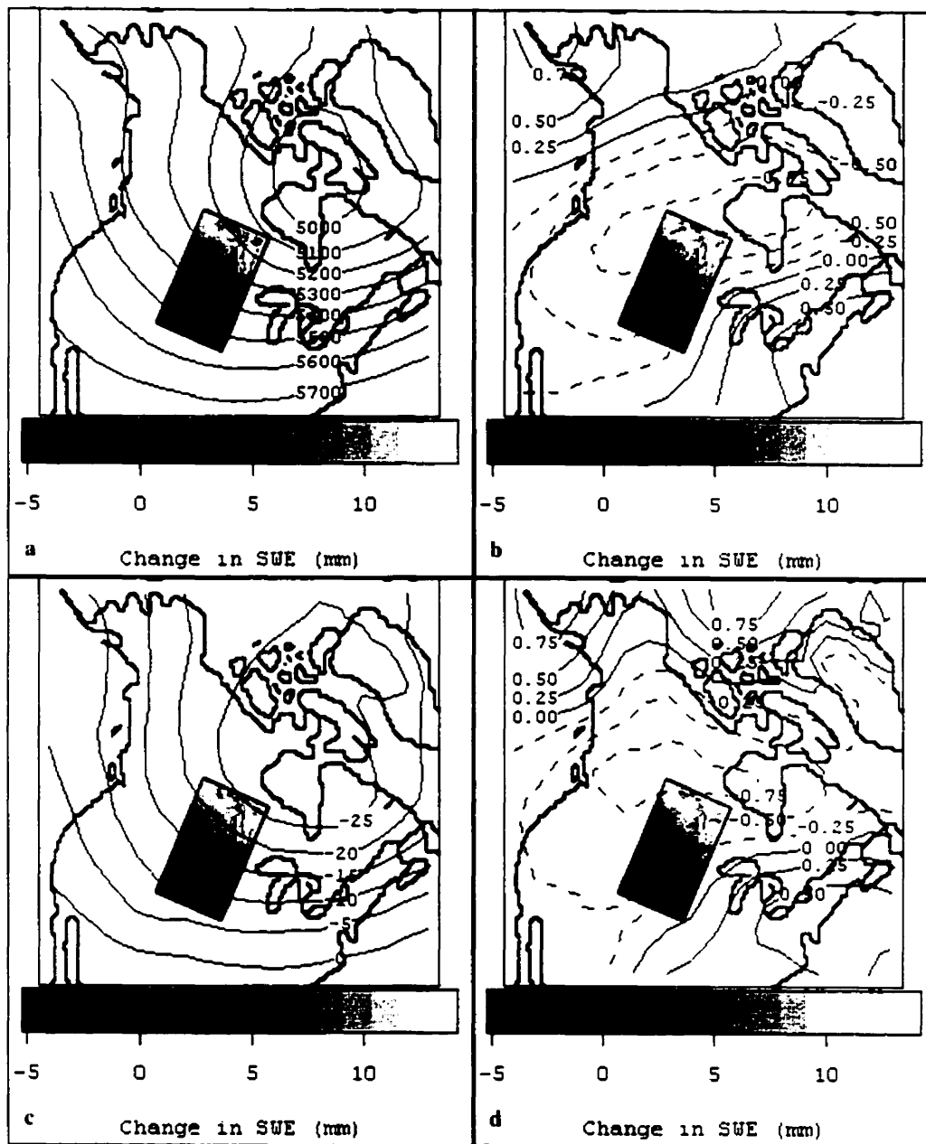
Figure 7.12 500Z composite (a) and anomaly (b), and 700T composite (c) and anomaly (d) fields, which correspond to the positive phase of \Delta SWE PC1 .
