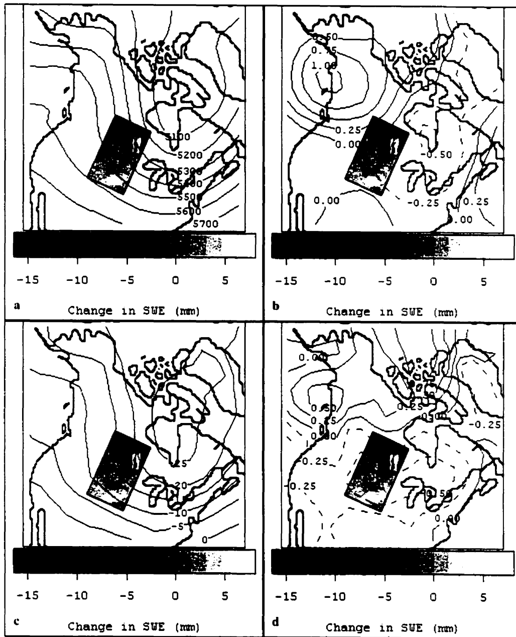
Figure 7.13 500Z composite (a) and anomaly (b), and 700T composite (c) and anomaly (d) fields, which correspond to the negative phase of \Delta\text{SWE PC1} .
