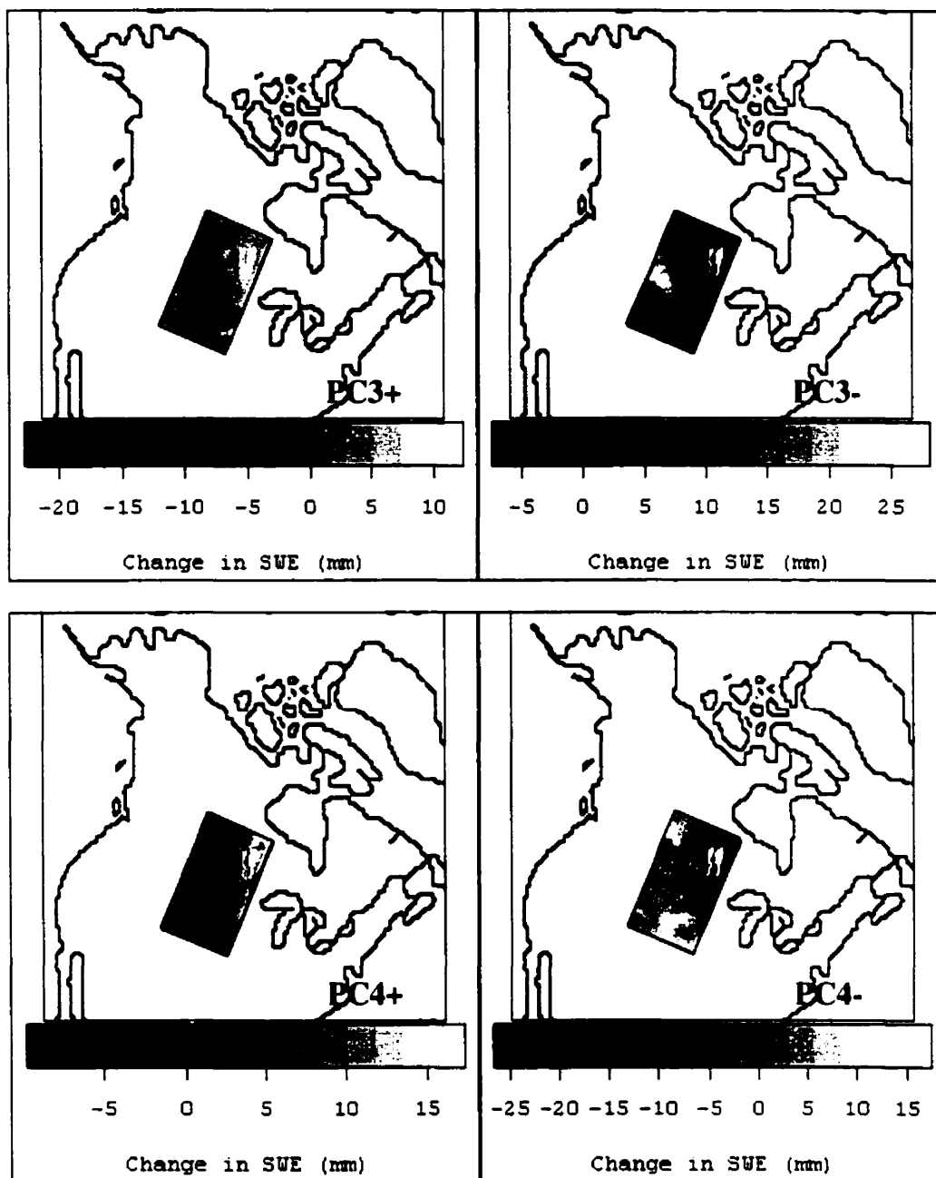
Figure 7.6 cont. Composite images which characterize the positive and negative phases of retained \Delta SWE components.
