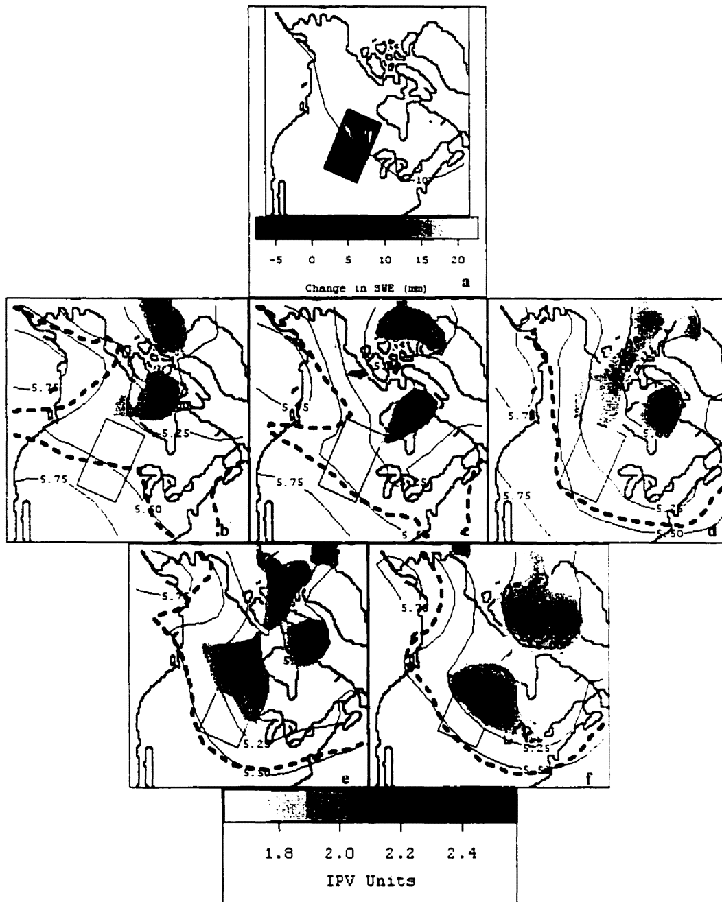
Figure 7.52 \Delta SWE PC2+ (shown in a with pentad average -10^{\circ}\text{C} isotherm at 700 mb) case study. Daily data for Feb. 25 ( b ) 1989 through March 1 ( f ) 1989 is shown. Gray tones illustrate IPV, the dashed line indicates the position of the -10^{\circ}\text{C} isotherm at 700 mb. solid lines depict the 500 mb geopotential height pattern (metres \bullet 10^3 ). \Delta SWE loading for this pentad is 0.77.
