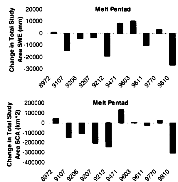
Figure 6.5 Change in total Prairie SWE (top) and SCA (bottom) for melt event pentads.
