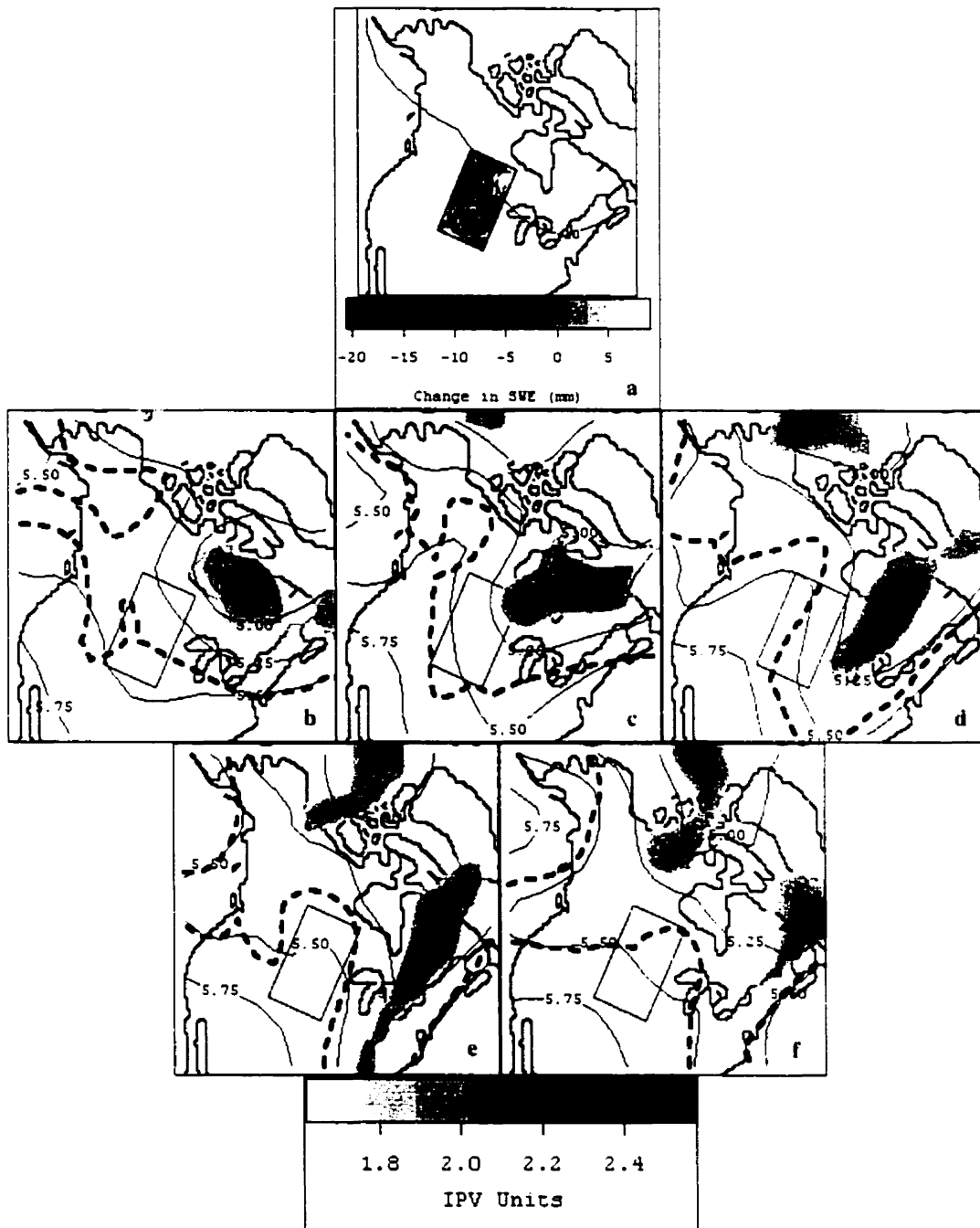
Figure 7.53 \Delta SWE PC2- (shown in a with pentad average -10^{\circ}\text{C} isotherm at 700 mb) case study. Daily data for Feb. 20 (b) 1989 through Feb. 24 (f) 1989 is shown. Gray tones illustrate IPV, the dashed line indicates the position of the -10^{\circ}\text{C} isotherm at 700 mb, solid lines depict the 500 mb geopotential height pattern (metres \times 10^3 ). \Delta SWE loading for this pentad is -0.58.
