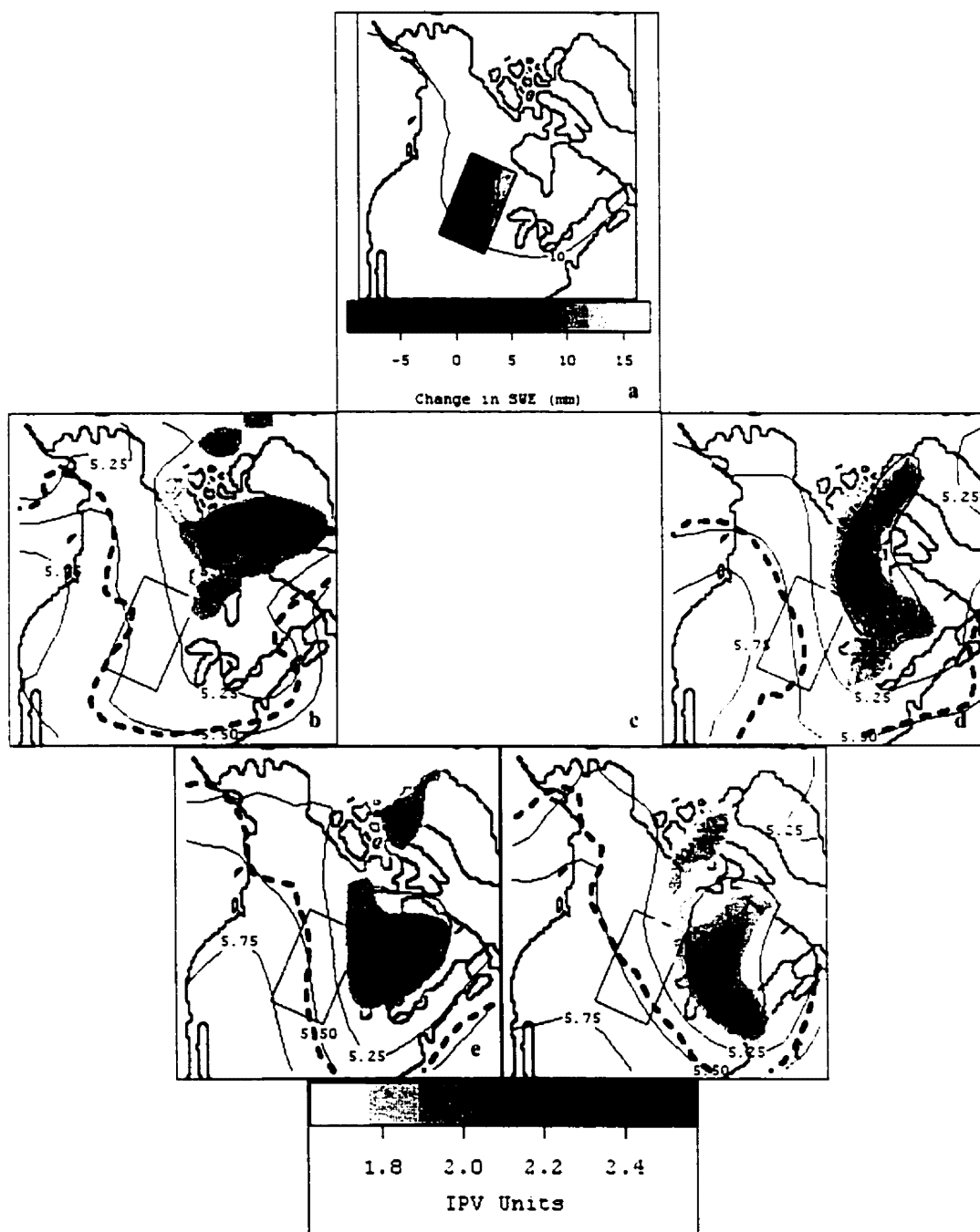
Figure 7.56 \Delta SWE PC4+ (shown in a with pentad average -10^{\circ}\text{C} isotherm at 700 mb) case study. Daily data for Dec. 22 ( b ) 1989 through Dec. 26 ( f ) 1993 is shown. Gray tones illustrate IPV, the dashed line indicates the position of the -10^{\circ}\text{C} isotherm at 700 mb, solid lines depict the 500 mb geopotential height pattern (metres \bullet 10^3 ). \Delta SWE loading for this pentad is 0.65.
