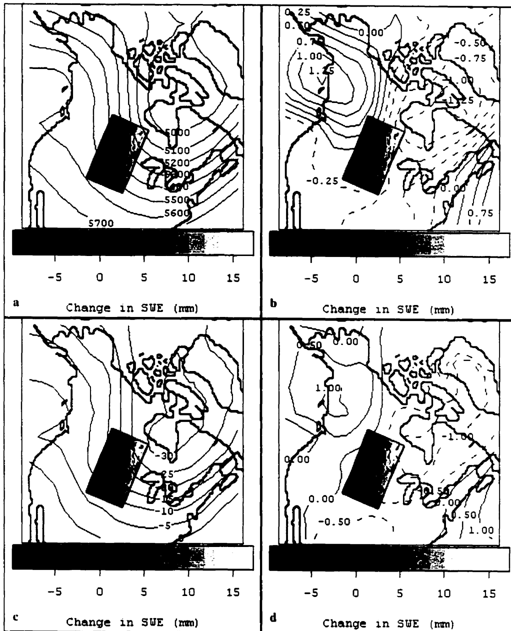
Figure 7.18 500Z composite (a) and anomaly (b), and 700T composite (c) and anomaly (d) fields, which correspond to the positive phase of \Delta\text{SWE PC4} .
