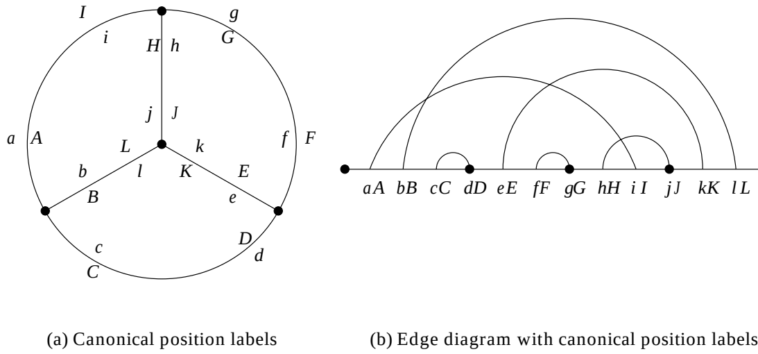
Figure 4.26: Linearising a rooted map into an edge diagram
