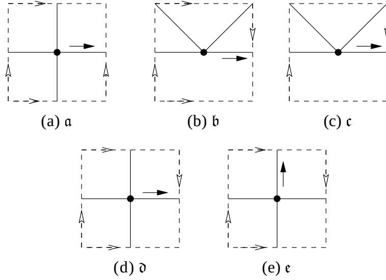
Figure 7.1: The five rooted maps \mathfrak{m} with \phi(\mathfrak{m}) = \nu(\mathfrak{m}) = [4]
