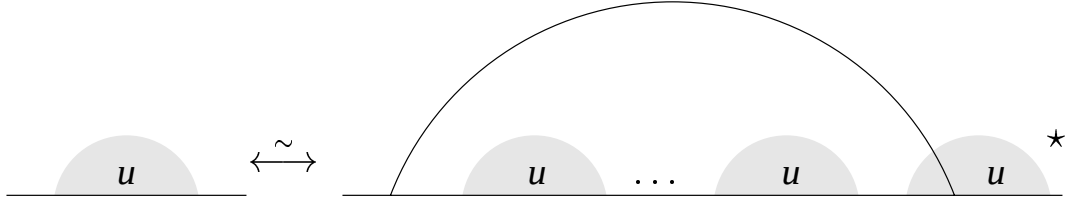
Figure 8.5: Ricatti decomposition for edge diagrams
