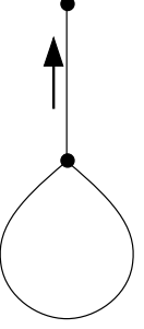
Figure 5.1: A planar rooted map \mathfrak{o} .
