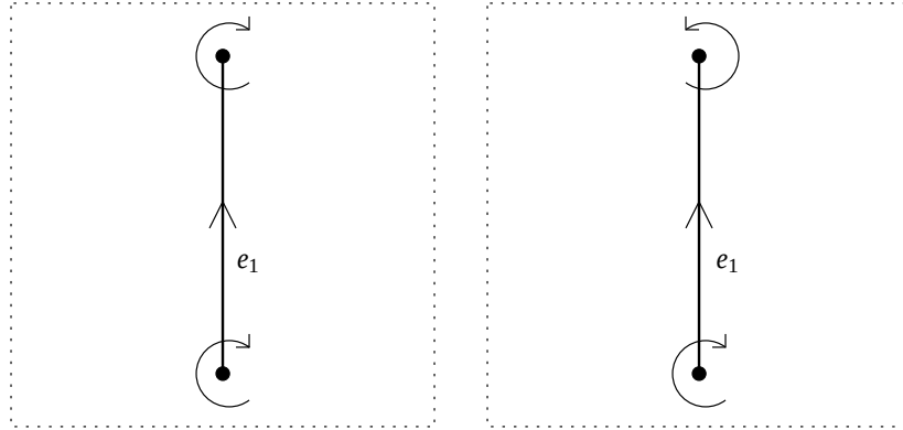
Figure 6.3: Both ordered digraphs of link deletion type
