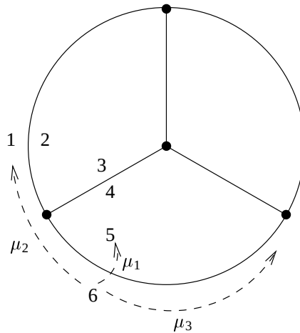
Figure 4.5: First instance that \mu_3 is used
