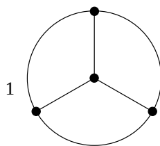
Figure 4.2: The algorithm begins at the root position
