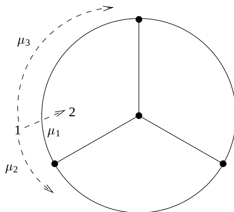
Figure 4.3: The algorithm moves along \mu_1 first
