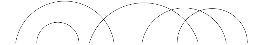
Figure 8.4: An unbroken arc configuration
