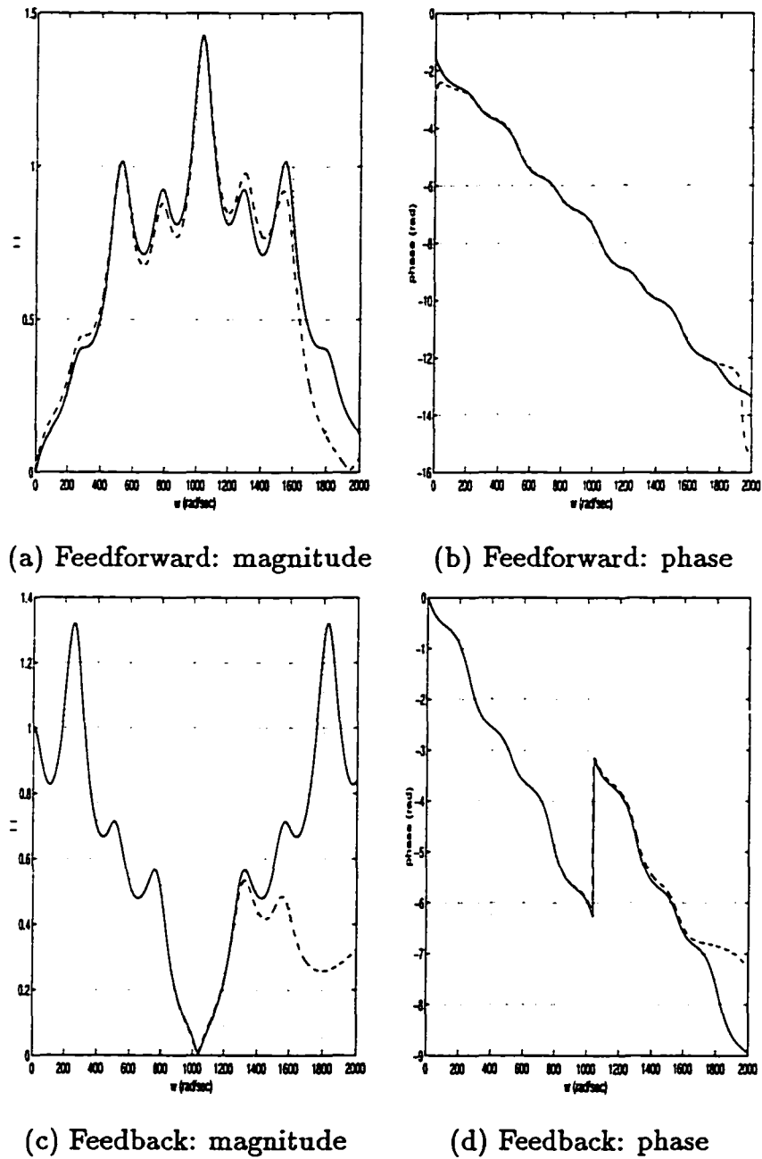
Figure 7.13: Legendre polynomials: feedforward and feedback (exact solution (solid), approximate solution for n = 10 (dashed))
