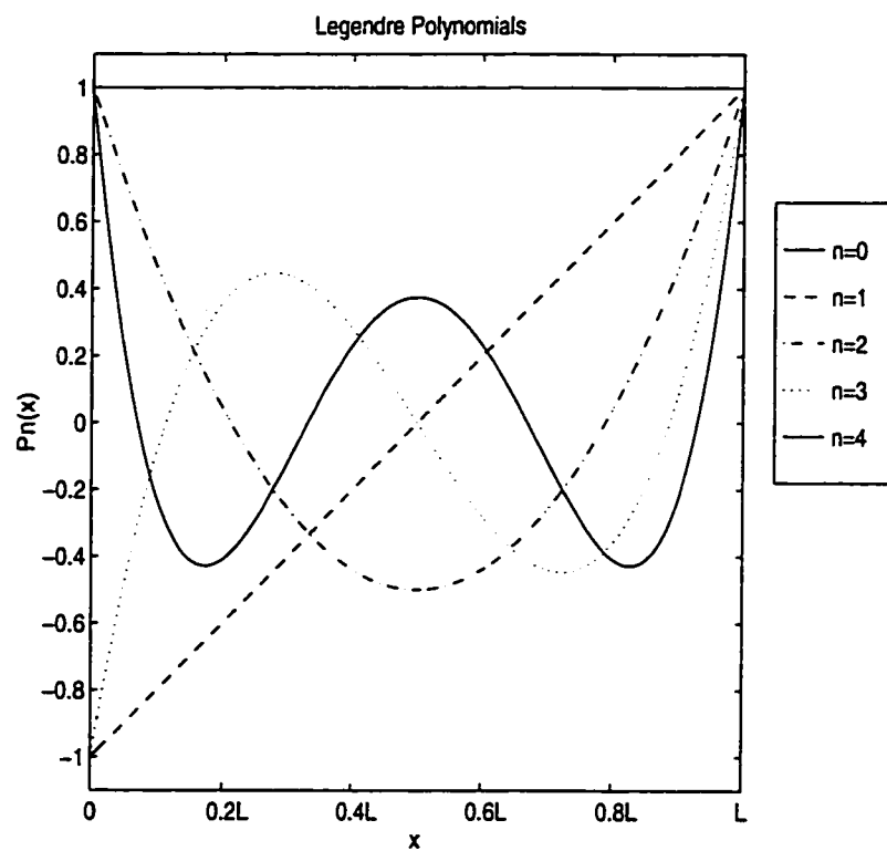
Figure 4.1: Legendre polynomials
