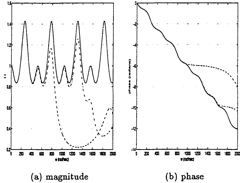
Figure 4.3: Legendre polynomials: magnitude and phase for G(jw) (solid) and G_n(jw) ( n = 5 (dashed), n = 10 (dash/dot))
