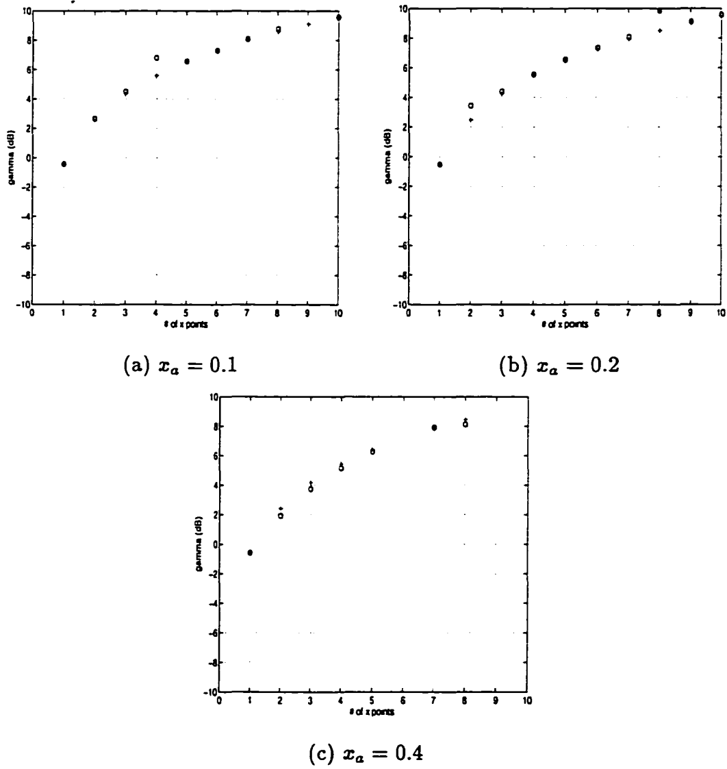
Figure 6.11: Dependence on m : x_s = 3 , bad x_a points ( \gamma (o), \gamma^{(1)}\sqrt{m} (+))
