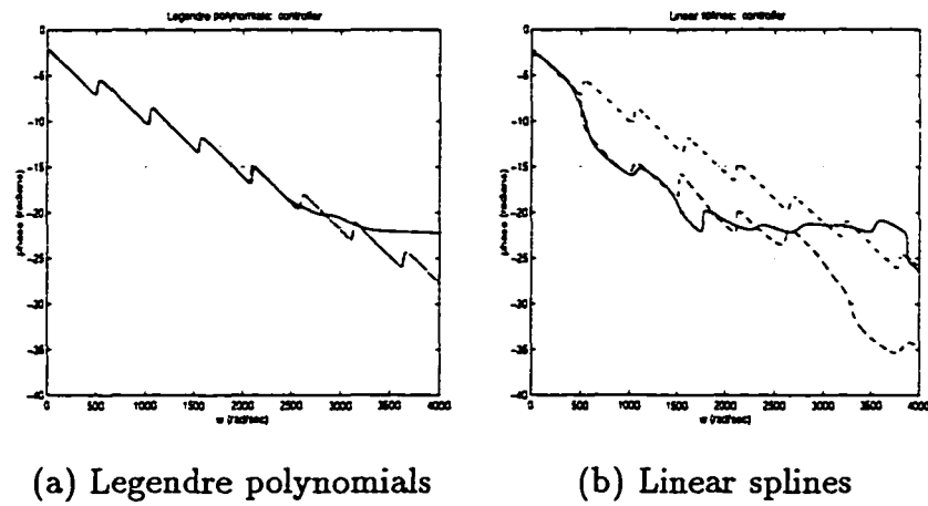
Figure 7.5: Case 1: phase of LQR controllers ( n = 15 (solid), n = 30 (dashed), n = 45 (dash/dot))
