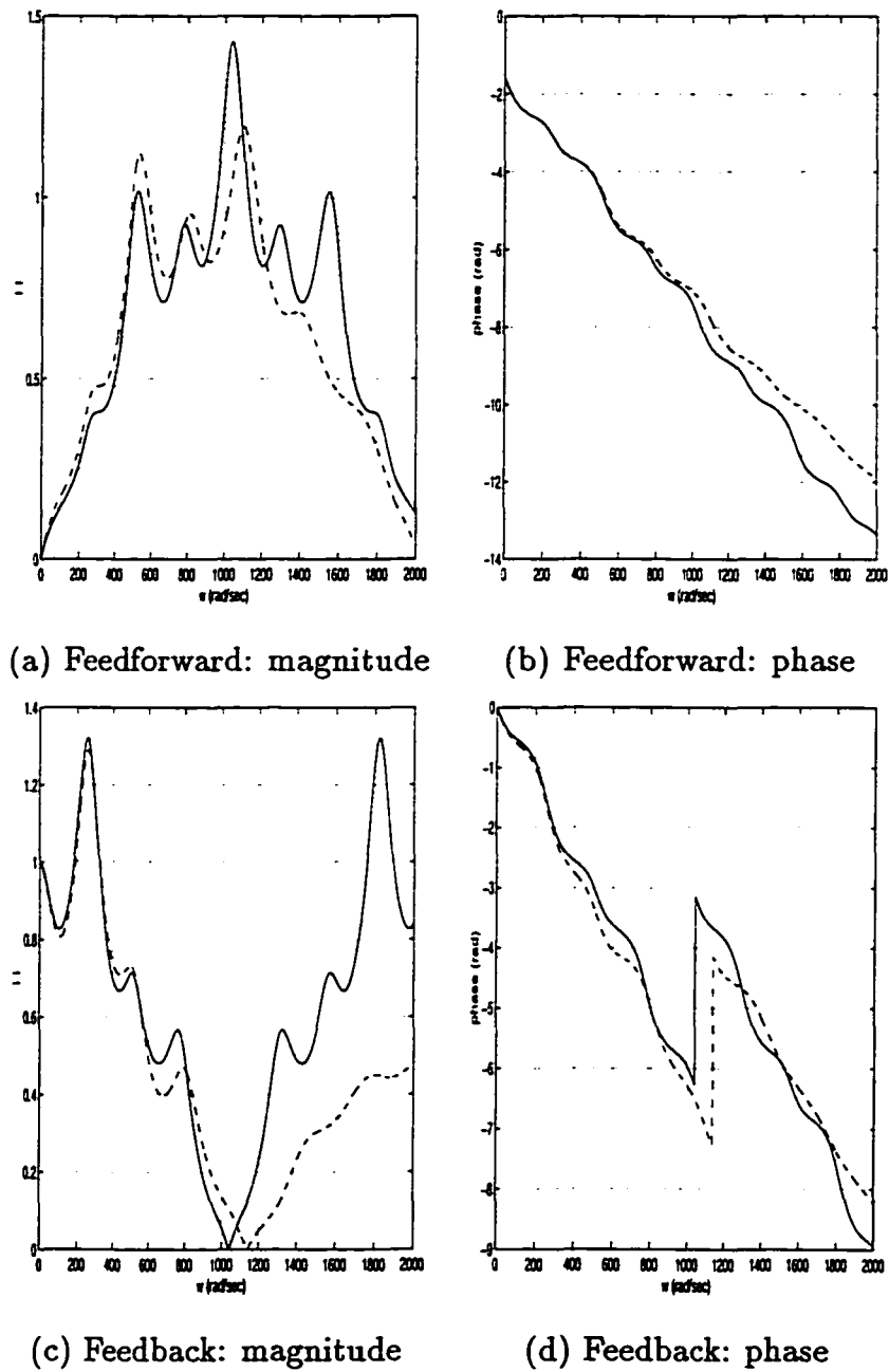
Figure 7.14: Linear splines: feedforward and feedback (exact solution (solid), approximate solution for n = 10 (dashed))
