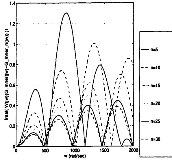
(a) |\Re[W_1(jw)(G_i(jw) - G_{n_i}(jw))]|
