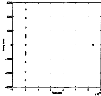
(e) zeros for n = 10
