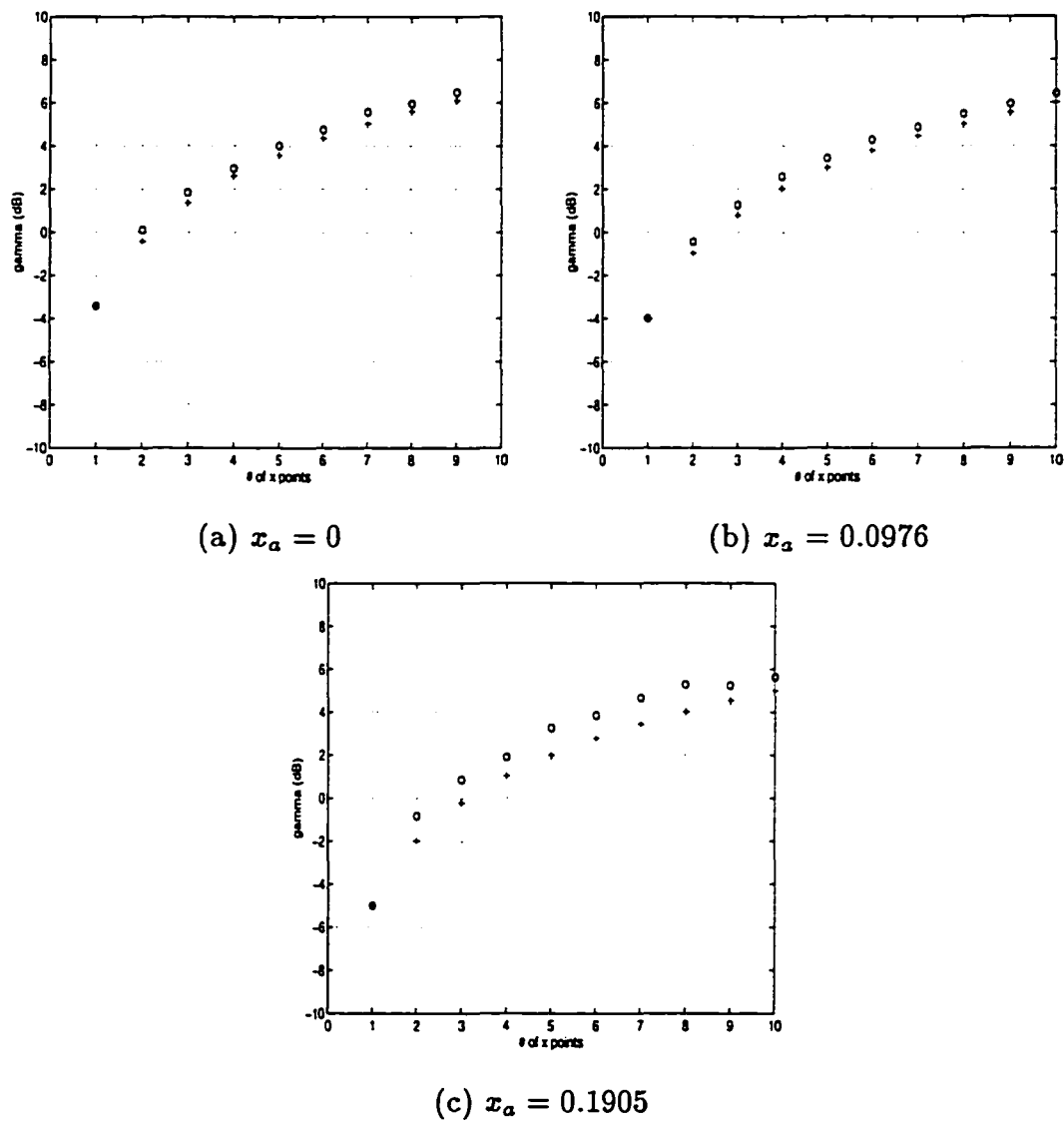
Figure 6.6: Dependence on m : x_s = 1 and good x_a points ( \gamma (o), \gamma^{(1)}\sqrt{m} (+))
