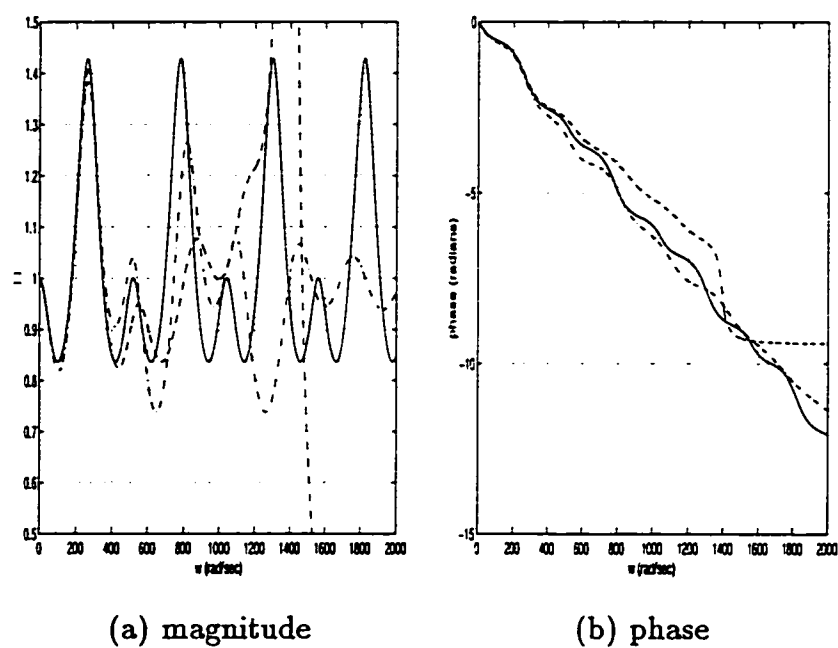
Figure 4.8: Linear splines: magnitude and phase for G(jw) (solid) and G_n(jw) ( n = 5 (dashed), n = 10 (dash/dot))
