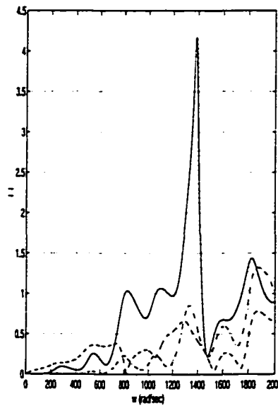
Figure 4.9: Linear splines: |G(jw) - G_n(jw)| ( n = 5 (solid), n = 10 (dashed), n = 15 (dash/dot))
