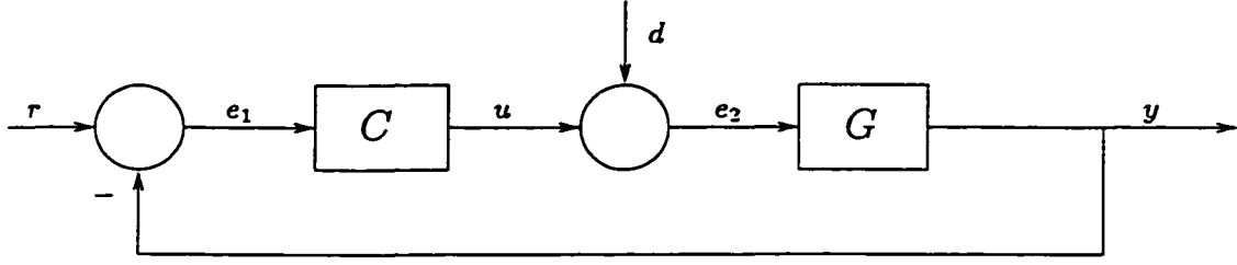
Figure 2.1: Basic feedback control system
