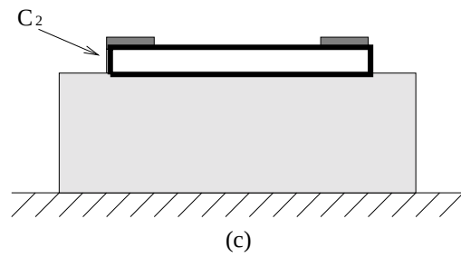
Figure 8.1: Diagram of a microstrip line structure with two narrow gold strips on the edges of the top surface of the HTSC strip and the specified surface C_1 and C_2
