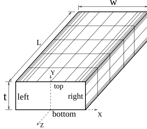
Figure 6.4: Diagram of a HTSC thin film with non-uniform gridding near the edges
