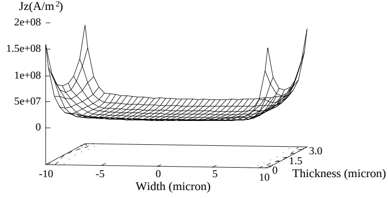
Figure 6.2: The J_z distribution of a thick superconducting film: w = 20\mu\text{m} , t = 3\mu\text{m} , h = 200\mu\text{m} , f = 1.5\text{GHz} , \lambda_L = 0.3\mu\text{m} .
