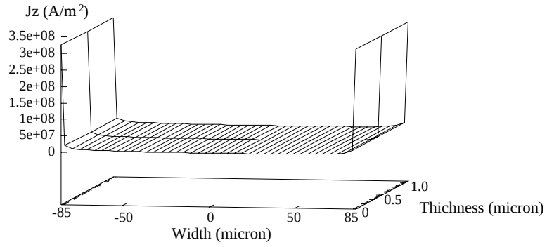
Figure 6.3: The J_z distribution of a thin superconducting film: w = 170\mu\text{m} , t = 1\mu\text{m} , h = 200\mu\text{m} , f = 1.5\text{GHz} , \lambda_L = 0.3\mu\text{m} .
