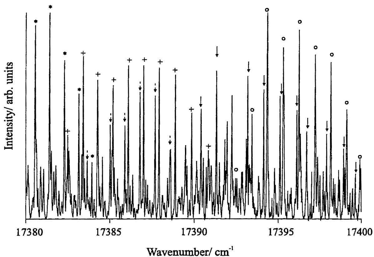
Figure 4.2: The resolved fluorescence spectrum of a portion of the R-branch of the \tilde{C}^2A_1-\tilde{X}^2A_1 transition of \text{CaNH}_2 . This spectrum was also recorded with a Broida oven but only the resolved fluorescence was monitored. This was done by placing the monochromator in the P-branch region of \tilde{C}^2A_1-\tilde{X}^2A_1 transition. The symbols denote lines belonging to a particular R-branch series, but matching the corresponding P-branch lines was impossible due to spectral congestion.
