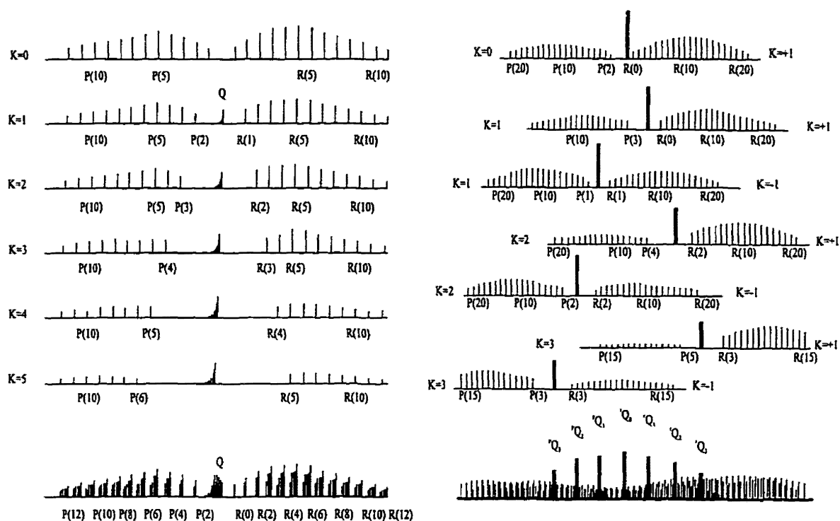
Figure 4.3: The comparison of the (a) parallel type and (b) perpendicular type transitions. The rotational contour of a parallel transition is much narrower than the contour of a perpendicular transition.
