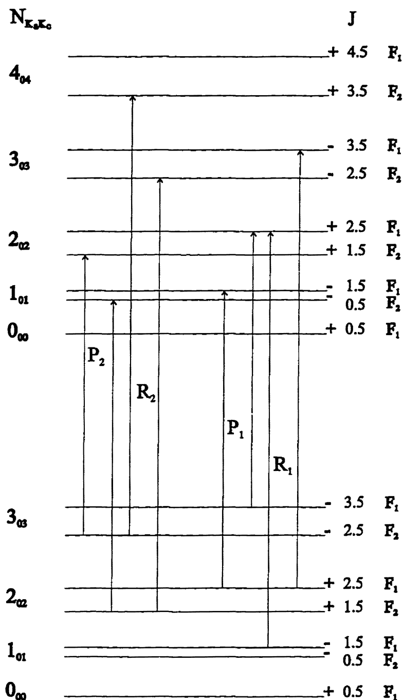
Figure 4.4: The energy level diagram associated with the K''_a = 0 \leftarrow K'_a = 0 sub-band of the \tilde{C}^2A_1 - \tilde{X}^2A_1 transition of \text{CaNH}_2 . The allowed transitions are labelled by \Delta J_{F_i} ( i = 1, 2 ).
