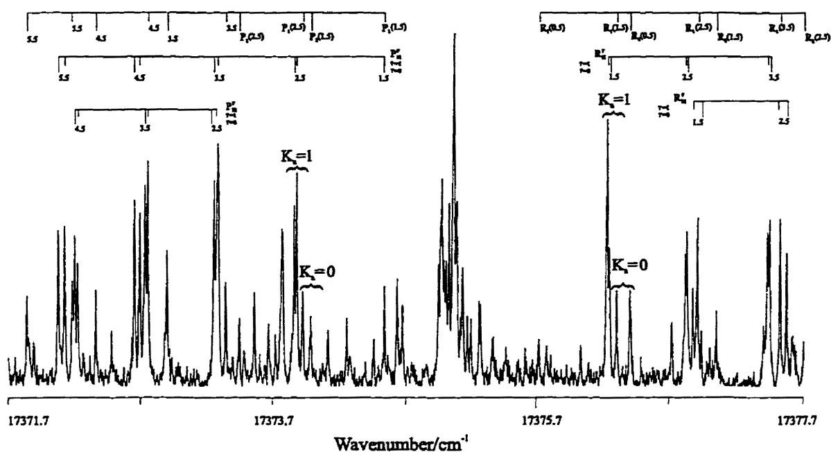
Figure 4.7: A portion of the high resolution spectrum of the 0_0^0 band of the \bar{C}^2A_1-\bar{X}^2A_1 transition of \text{CaNH}_2 near the origin. This spectrum was recorded with He carrier gas. Note the 3:1 intensity ratio of ortho ( K_a = 1 ) and para ( K_a = 0 ) levels and the small asymmetry splitting ( \gamma ) of the K_a'' = 1 \leftarrow K_a' = 1 sub-band. The Q-branch transitions are not labelled for clarity.
