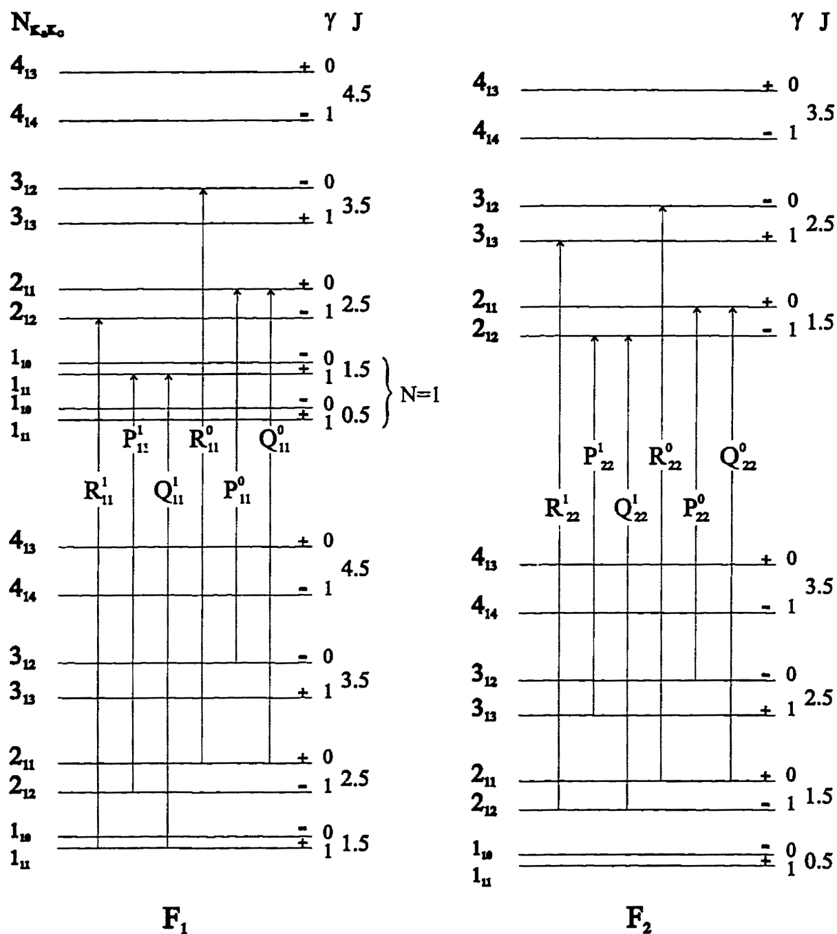
Figure 4.5: The allowed transition of the K'' = 1 \leftarrow K' = 1 sub-band of the \tilde{C}^2A_1 - \tilde{X}^2A_1 transition. Each transition is labelled by \Delta J''_{F'', F'} ( i = 1, 2 ), see text for details.
