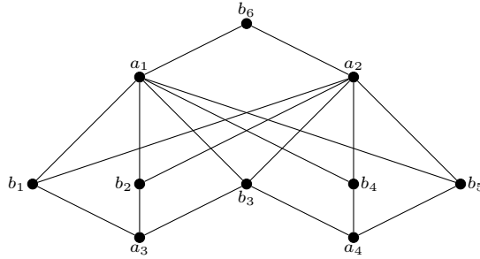
Fig. 13. For the proof of 6.1.
