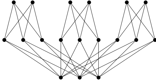
Fig. 1. Counterexample to 2.1 with t = 5 .
