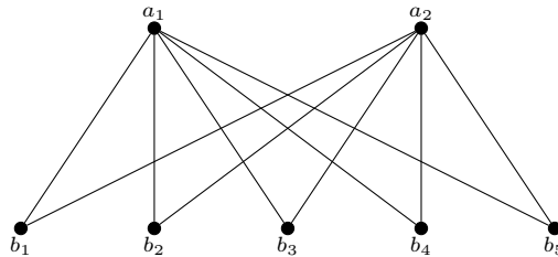
Fig. 14. K(2, 5, 0) -subgraph.
