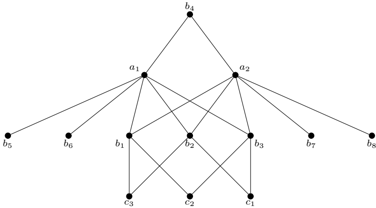
Fig. 24. For the proof of 8.2.
