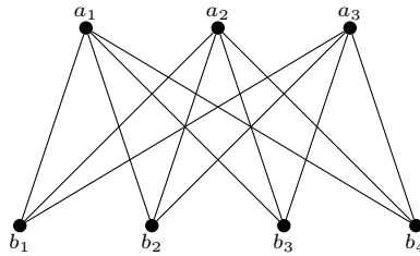
Fig. 10. K(3, 4, 0) -subgraph.
