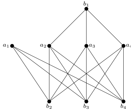
Fig. 8. K(4, 4, 1) -subgraph.
