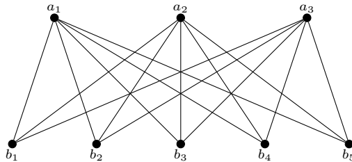
Fig. 4. K(3, 5, 0) -subgraph.
