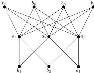
Fig. 9. K(3, 7, 3) -subgraph.
