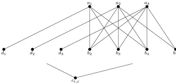
Fig. 21. The start of the proof of 8.1. c_{i,j} is adjacent to d_i and b_j .
