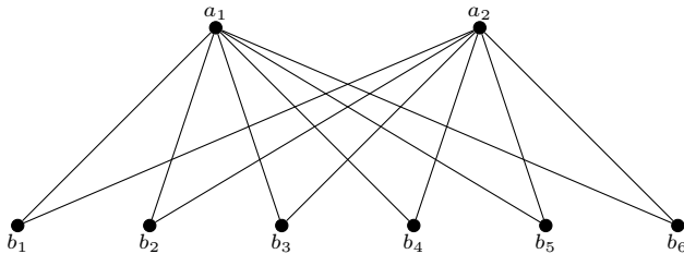
Fig. 12. K(2, 6, 0) -subgraph.
