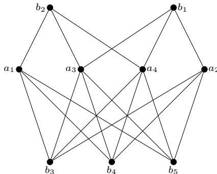
Fig. 7. K(4, 5, 2) -subgraph.
