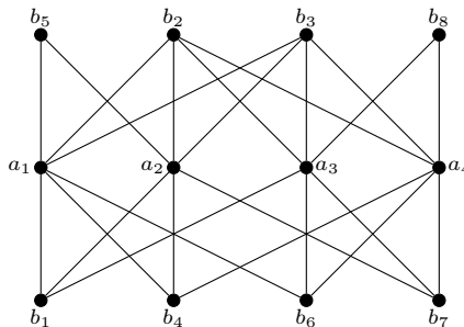
Fig. 17. For the last part of the proof of 6.2. ( a_5 is not drawn.)
