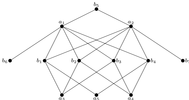
Fig. 15. For the proof of 6.2.
