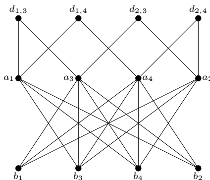
Fig. 19. For the proof of 7.1, step (2).
