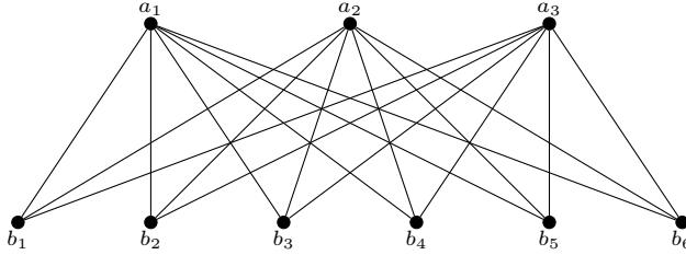
Fig. 3. K(3, 6, 0) -subgraph.
