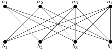
Fig. 2. K(4, 4, 0) -subgraph.
