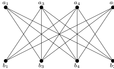
Fig. 18. K(4, 4, 2) -subgraph.
