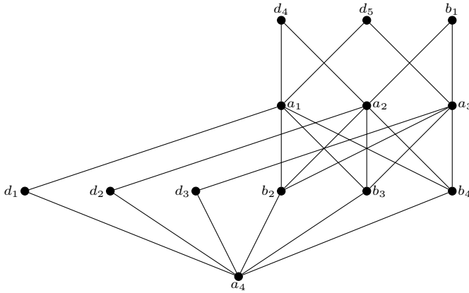
Fig. 23. For the last part of the proof of 8.1.
