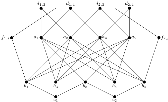
Fig. 20. For the last part of the proof of 7.1. f_{1,i} is adjacent to d_{1,i} for some i \in \{3, 4\} , and similarly for f_{2,j} . The vertices c_1, c_2 might be equal, but f_{1,i} is different from f_{2,j} .
