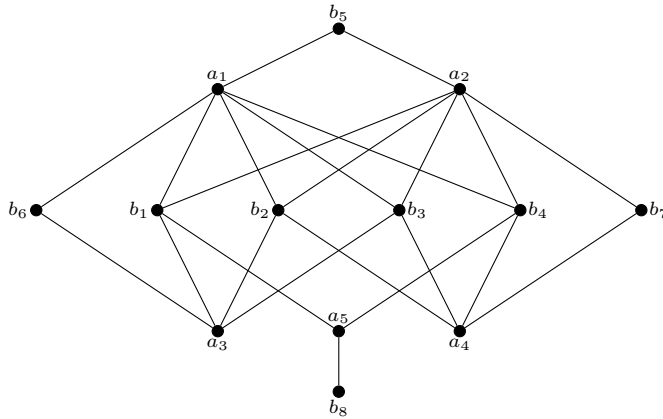
Fig. 16. For the proof of 6.2, step (6).
