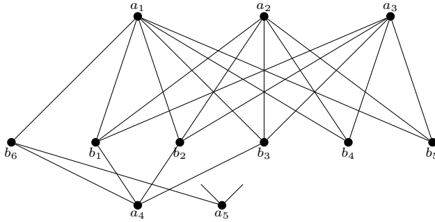
Fig. 5. For the last part of the proof of 4.3. a_5 is adjacent to two of b_1, \dots, b_5 .
