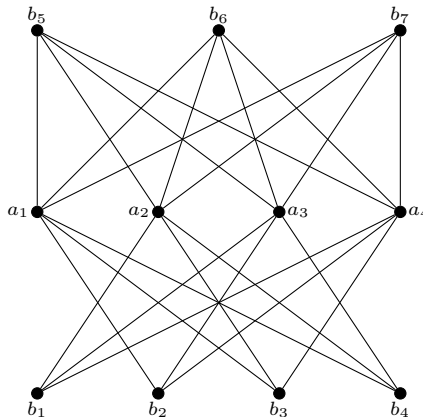
Fig. 6. K(4, 7, 4) -subgraph.
