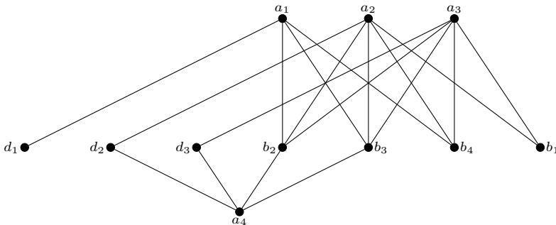
Fig. 22. For the proof of 8.1, step (4).
