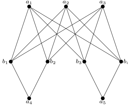
Fig. 11. For the proof of 5.2.
