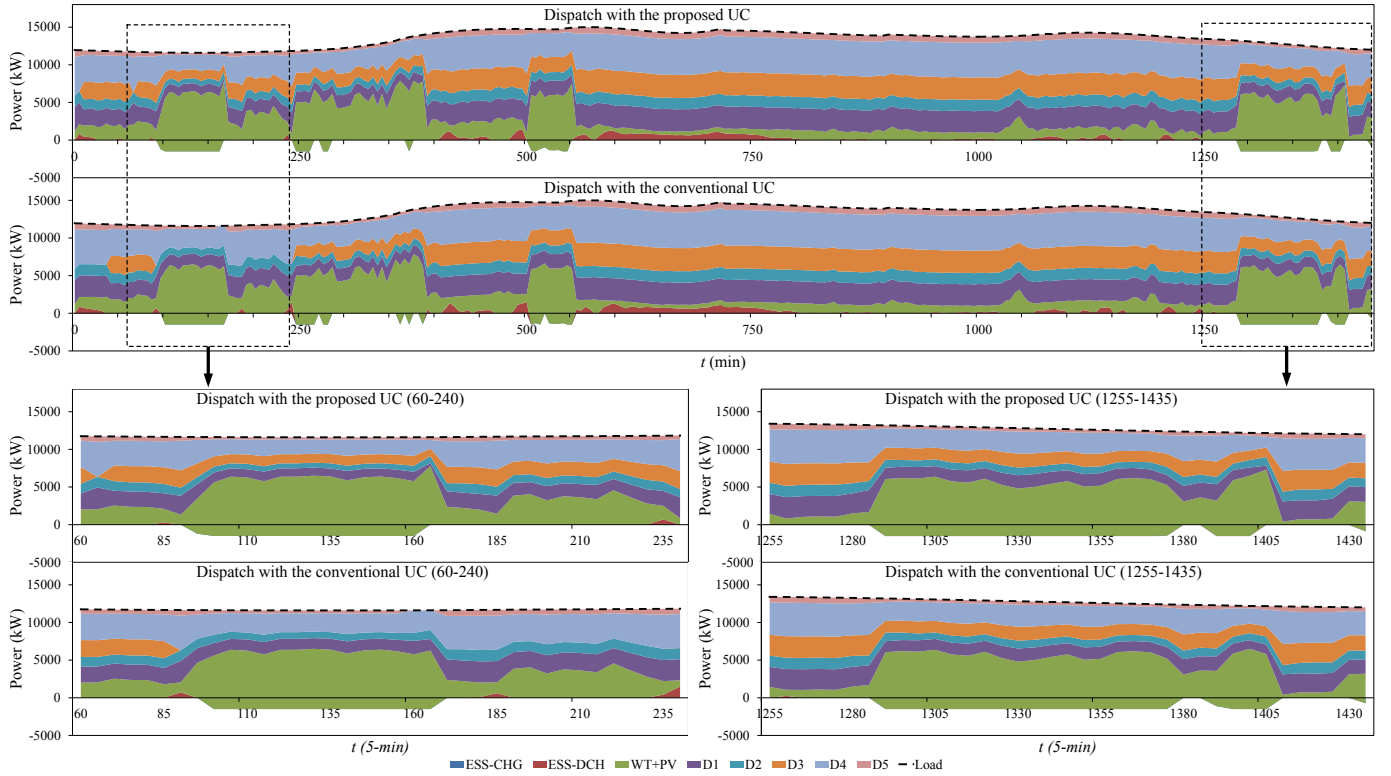
Fig. 10. Case D dispatch results with the proposed and conventional UC.
