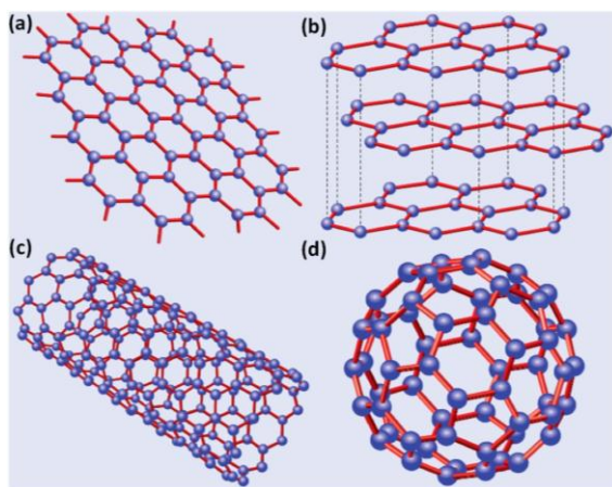
Figure 2.1. a) Graphene (a honeycomb lattice of carbon atoms). b) Graphite (a stack of graphene layers). c) Carbon nanotube (a rolled-up cylinder of graphene). d) Fullerene (a molecule consisting of wrapped graphene) [Courtesy of APS publications with permission] [43].
