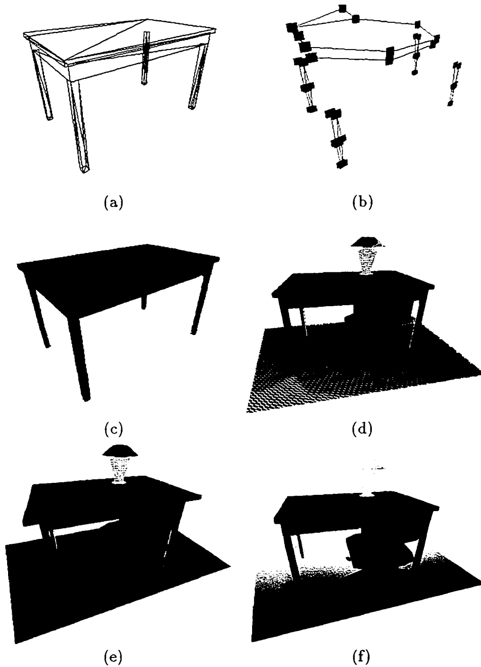
Figure 4.21: Experiments on the augmented reality of a laboratory table: (a) the triangular mesh model of the table; (b) the AHR of the table constructed from the triangular mesh; (c) the reconstructed geometry with colors and textures of the table; (d) the augmented scene with textured floor, a table lamp and an arm chair; (e) enlarged table top; (f) the table with marble top and virtual lighting effects.
