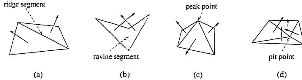
Figure 3.11: Geometrical features in triangular meshes: (a) ridge line segment; (b) ravine line segment; (c) peak point; (d) pit point.
