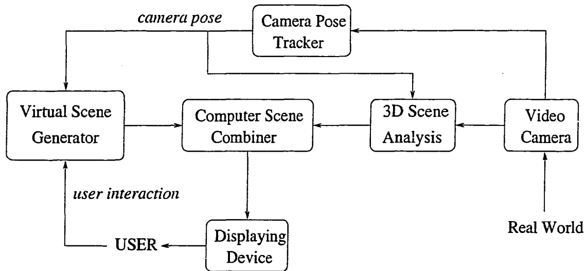
Figure 2.2: Improved see-through device with computer aided video combination for augmented reality.
