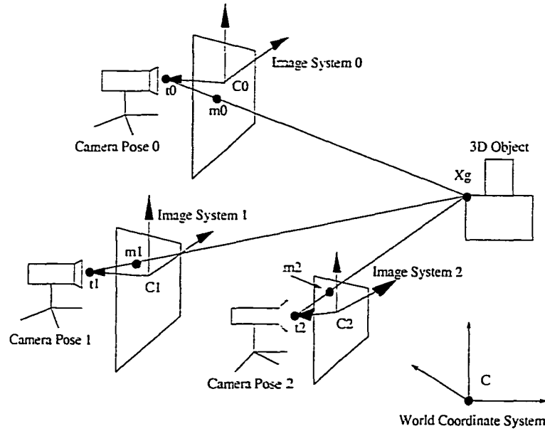
Figure 4.1: The multiple-view system for 3D model synthesis.
